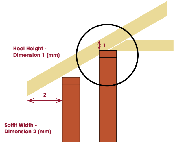
Figure 4. Option 2: Truss Roof Eaves
