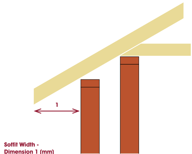
Figure 4. Option 2: Truss Roof Eaves
