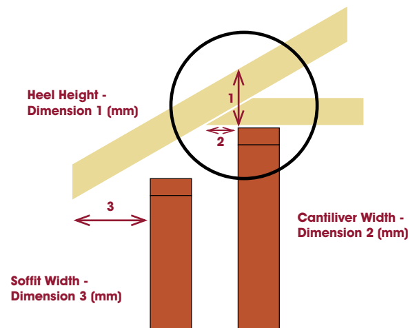
Figure 4. Option 3: Modified Truss Eaves
